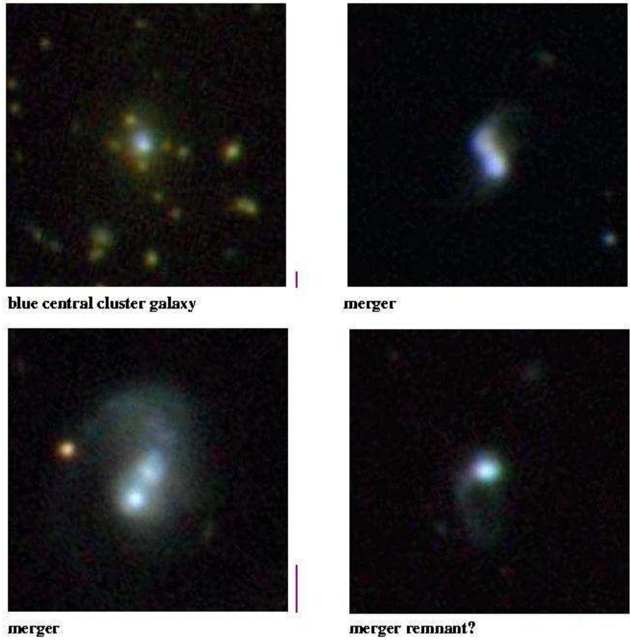
Figure 25: A montage of 48'' \times 48'' images of AGN with [OIII] luminosities greater than 10^{7.8} L_{\odot} .
